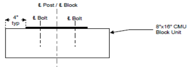
CMU BLOCK - PLATE CONNECTION DETAIL
