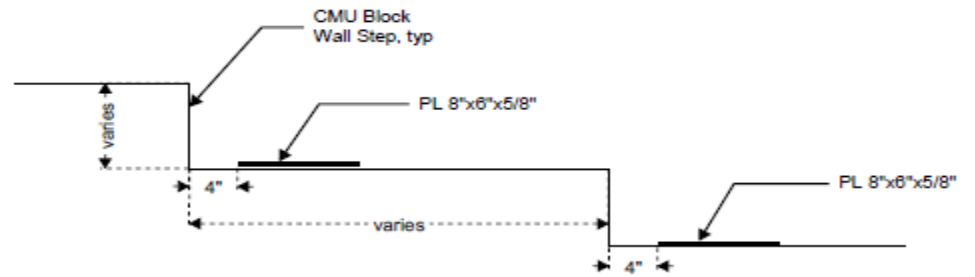
ELEVATION DETAIL - RAILING CONNECTION
