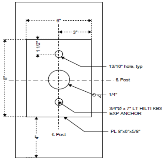
PLAN DETAIL - RAILING CONNECTION
